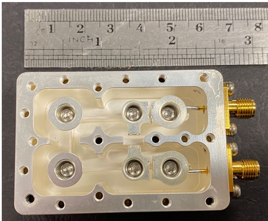
Figure 11: Hardware realization of an order 6 filter in combline technology
