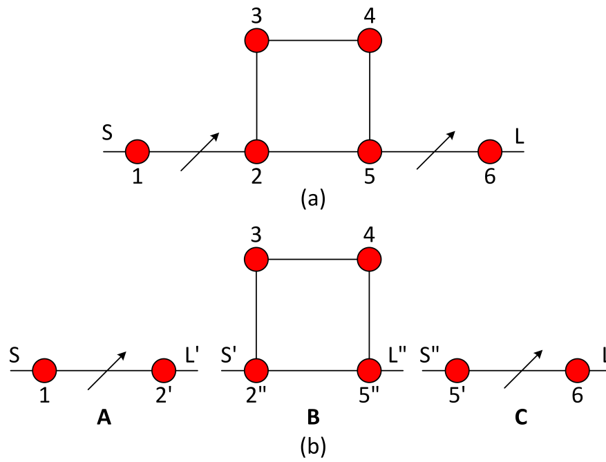
Figure 10: a: Topology combining a quadruplet and two sections with dispersive couplings - b: circuitual blocs associated to the functional decomposition
