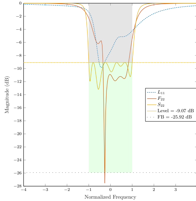
Figure 9: Reflection coefficients: L_{11} antenna, S_{22} global system, F_{22} matching circuit. FB is the Fano bound.
