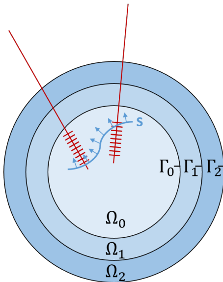
Figure 6: Spherical 3 layered head, schematic view. Deep electrodes with sensors along them (red) in \Omega_0 , current source term \mu distributed on S \subset \Omega_0 with normally oriented dipoles.
